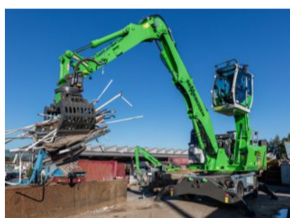
Sennebogen 817M-E Electro Battery
